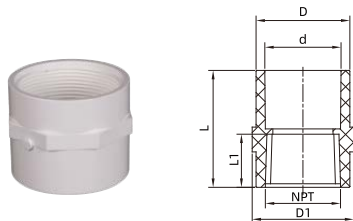
Female Adaptor
