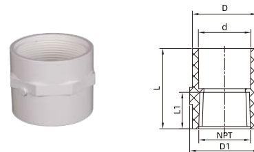
Female Adaptor
